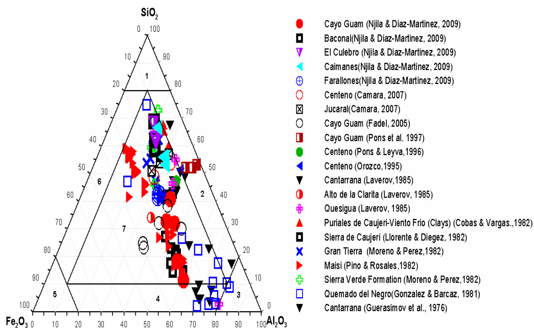
Figure 1. \text{SiO}_2\text{-Al}_2\text{O}_3\text{-Fe}_2\text{O}_3 plot for the non-nickeliferous weathering crust in Eastern Cuba. 1- silicic; 2- sialitic; 3- allitic; 4- ferrallitic; 5- ferric; 6- ferrisilicic; 7- ferrosialitic.
